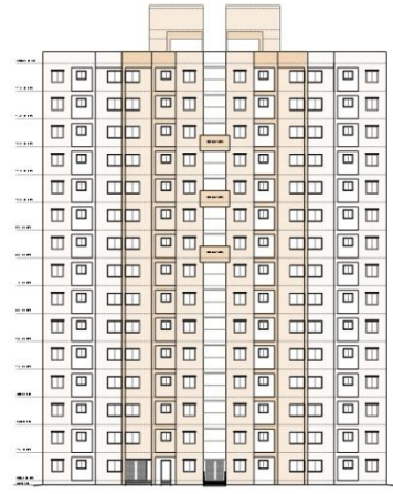
FRONT ELEVATION
